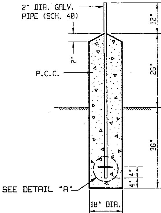
SECTION "X"-"X"
