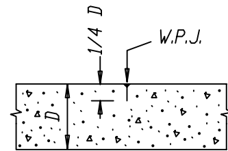
TYPICAL W.P.J. SECTION NOT TO SCALE
