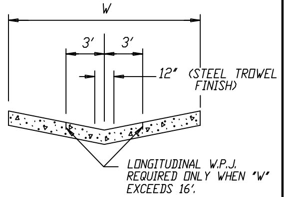
TYPICAL PAVEMENT SECTION NOT TO SCALE
