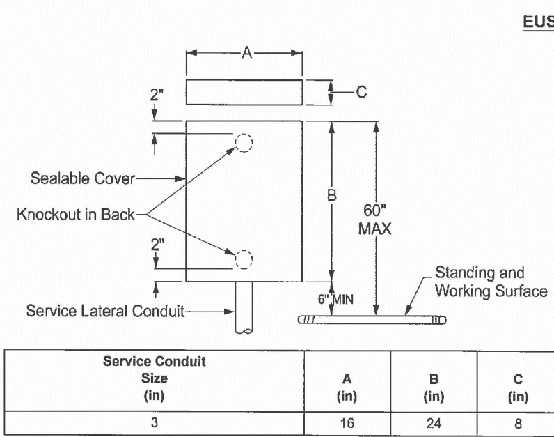
Figure 3-11: Underground Pull Boxes
