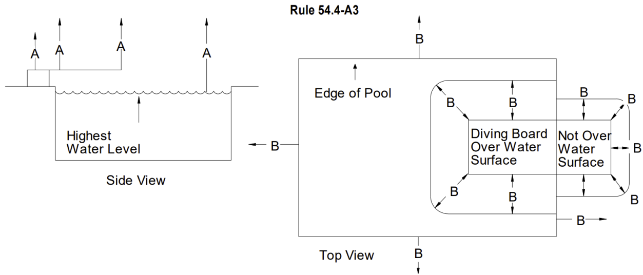
Clearance Over Swimming Pools Figure 54-1
