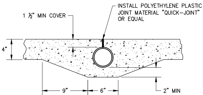
SECTION A-A RESIDENTIAL
