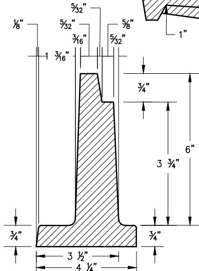
DETAIL OF FRAME
