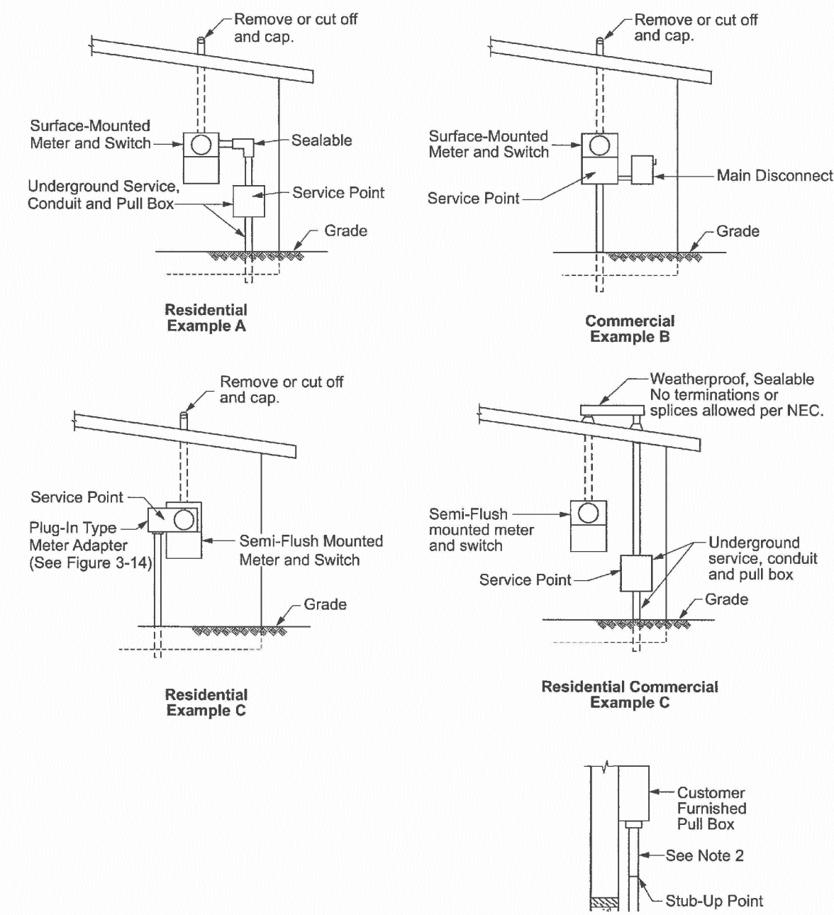
Figure 3-13: Typical Service Conversion from Overhead to Underground
